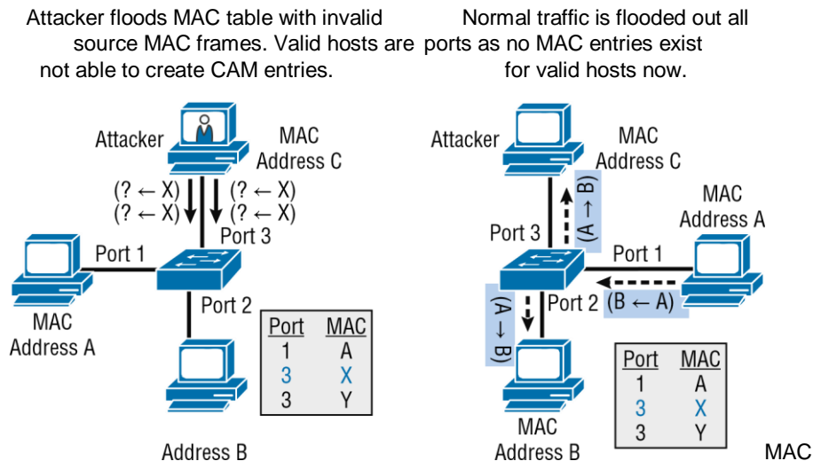
FIGURE 11.21 Flood guard process
