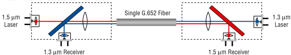
FIGURE 3.9 Bidirectional communication
