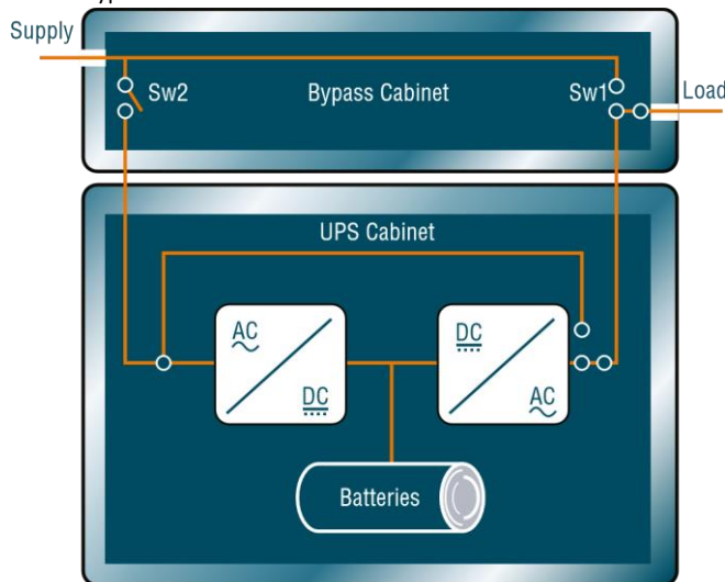
FIGURE 13.8 Maintenance bypass
