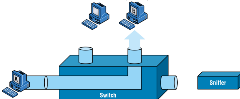
FIGURE 11.26 Switches send frames out the destination port only.
