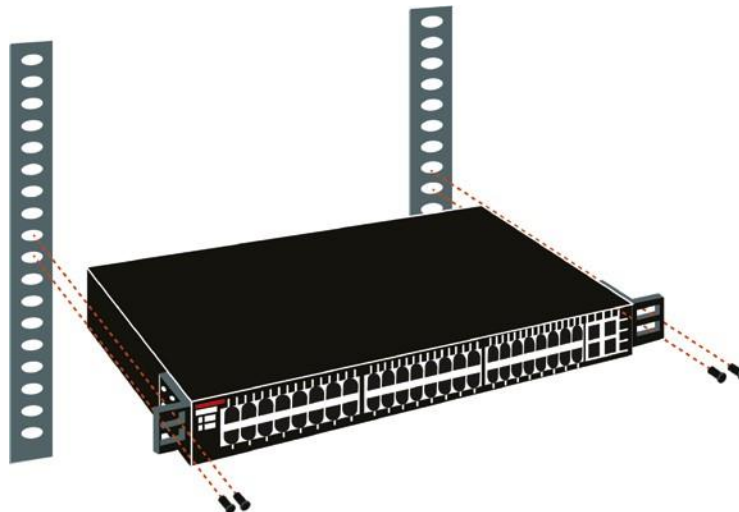
FIGURE 21.14 Rack- mounted switches
