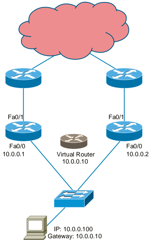
FIGURE 15.6 FHRPs use a virtual router with a virtual IP address and virtual MAC address.
