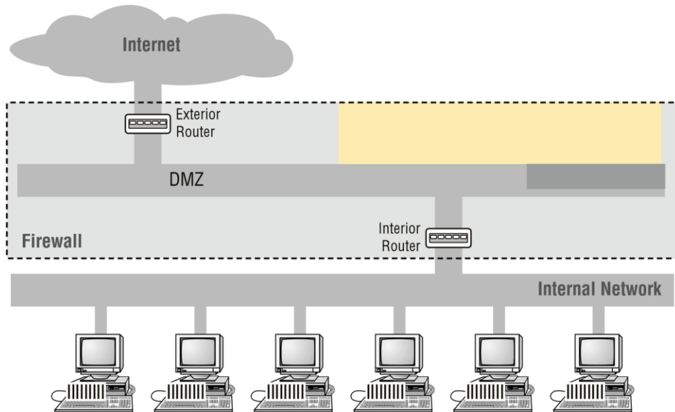
FIGURE 16.1 Screened subnet
