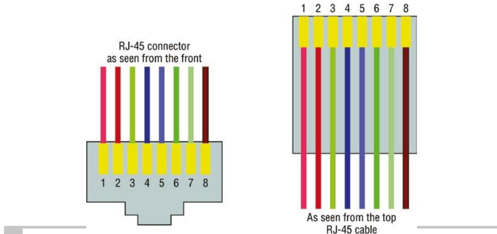
FIGURE 21.13 Two ends of a crossover cable
