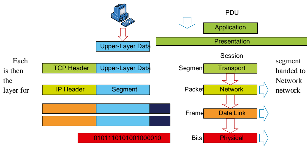
FIGURE 6.21 Data encapsulation
