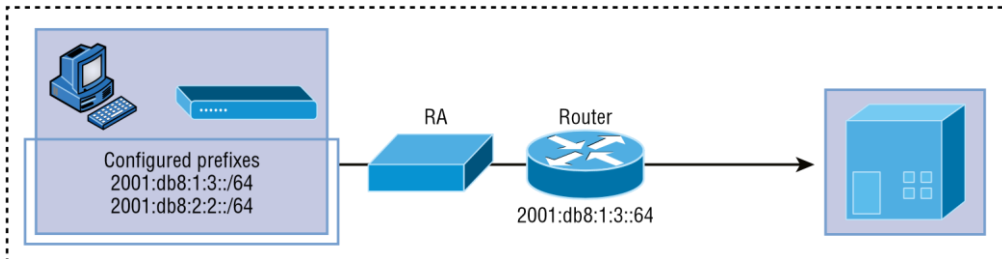
FIGURE 18.1 RA Guard
