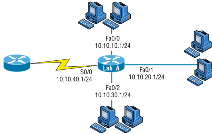
FIGURE 9.1 A simple routing example
