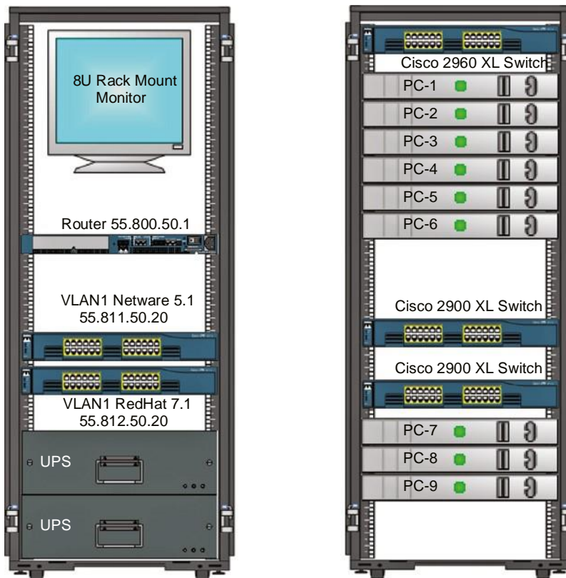
FIGURE 14.4 Hardware- rack diagram from SmartDraw
