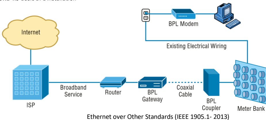
FIGURE 4.9 Basic BPL installation
