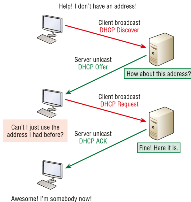
FIGURE 6.7 DHCP client four-s tep process
