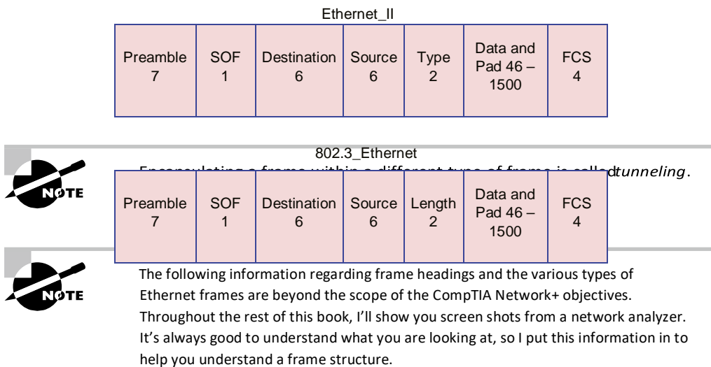
FIGURE 4.6 802.3 and Ethernet frame formats in bytes
