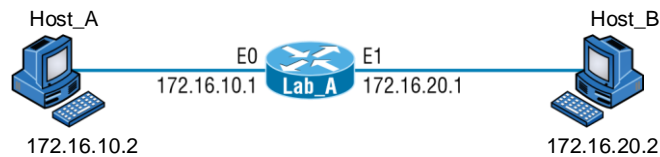
FIGURE 9.2 IP routing example using two hosts and one router
