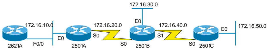
FIGURE 10.2 The internetwork with distance- vector routing
