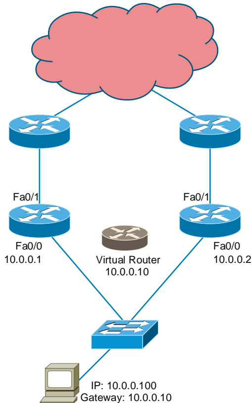
FIGURE 10.11 FHRPs use a virtual router with a virtual IP address and virtual MAC address.
