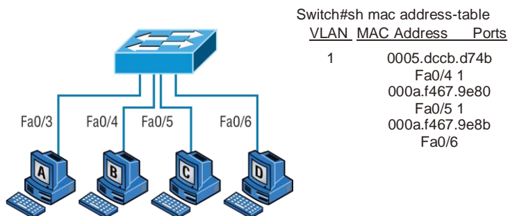
FIGURE 11.7 Forward/filter table
