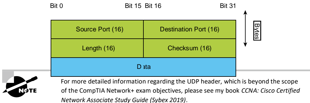
FIGURE 6.13 UDP segment
