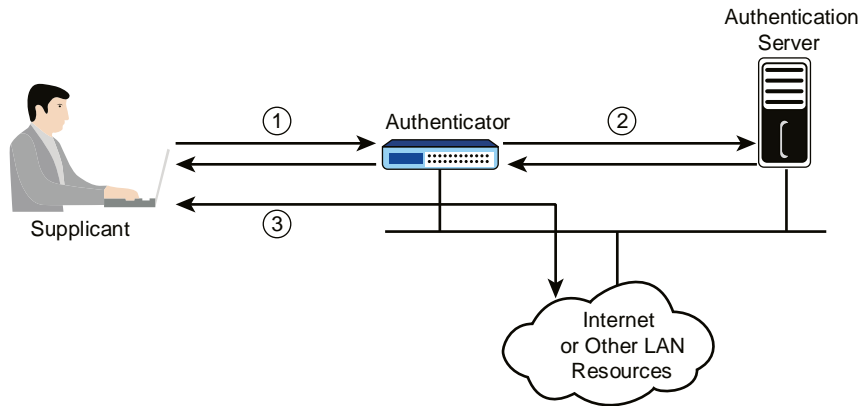
FIGURE 16.4 802.1X
