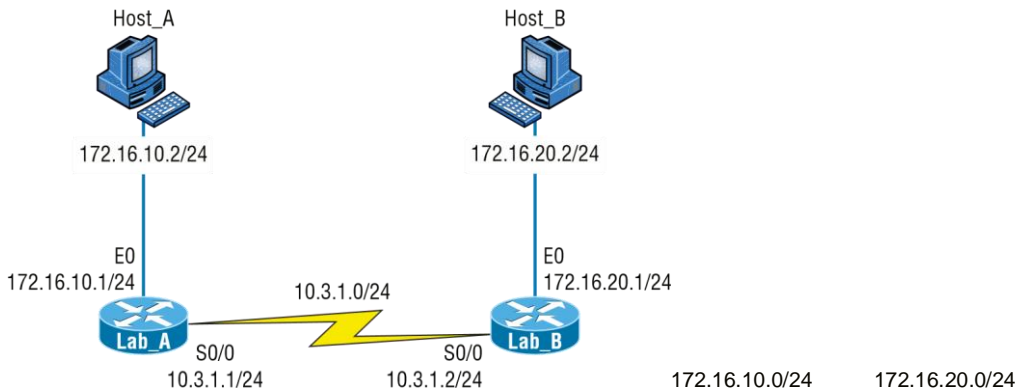
FIGURE 10.6 A discontinuous network
