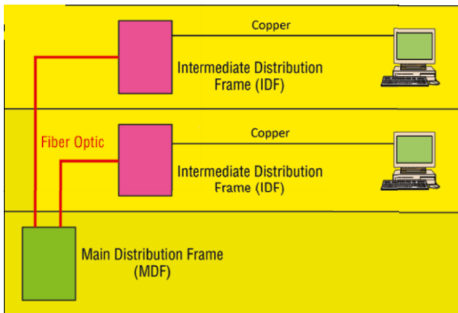
FIGURE 21.22 MDF and IDFs
