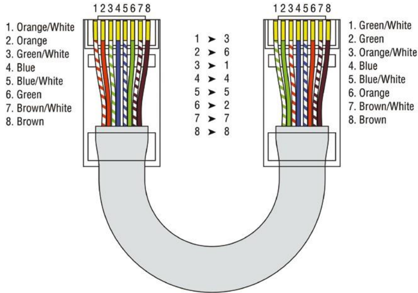
FIGURE 21.12 RJ-45 connector
