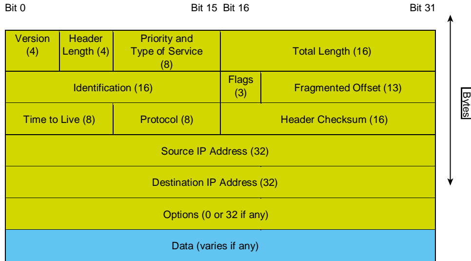
FIGURE 6.15 IPv4 header
