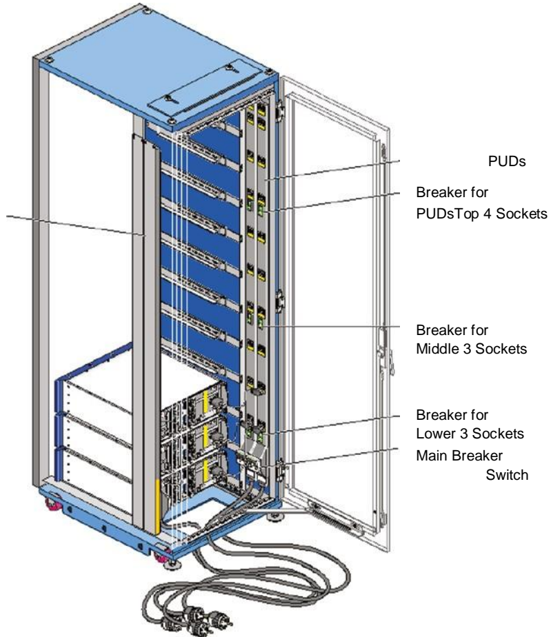
FIGURE 13.9 Multiple circuits
