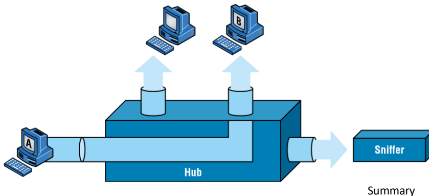
FIGURE 11.27 Place a hub between two hosts to troubleshoot.
