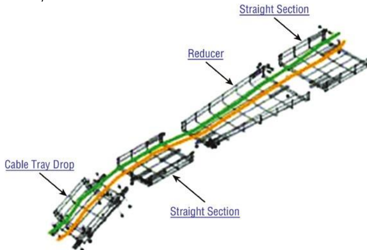
FIGURE 21.23 Cable trays
