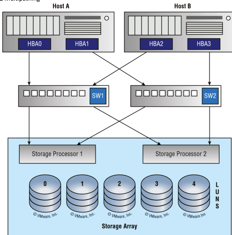
FIGURE 15.1 Multipathing
