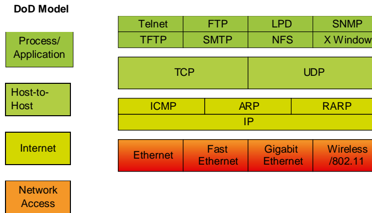
FIGURE 6.2 The TCP/IP protocol suite
