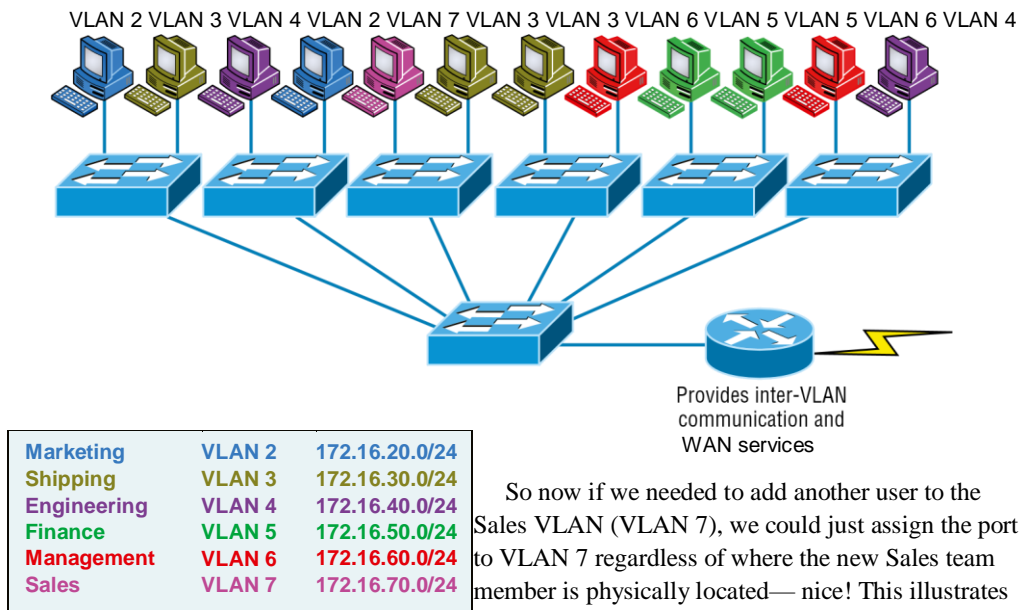
FIGURE 11.16 Switches removing the physical boundary
