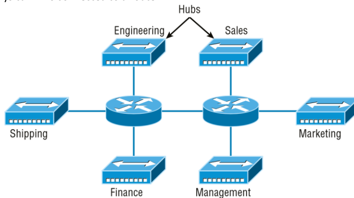
FIGURE 11.15 Physical LANs connected to a router
