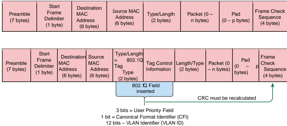
FIGURE 11.18 IEEE 802.1Q encapsulation with and without the 802.1Q tag
