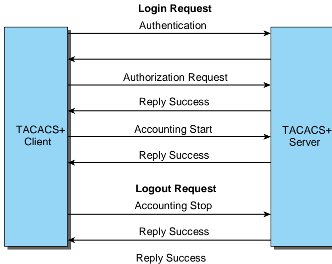
FIGURE 16.2 TACACS+ login and logout sequence
