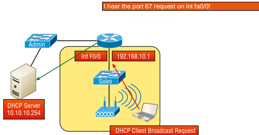
FIGURE 5.13 Configuring a DHCP relay
