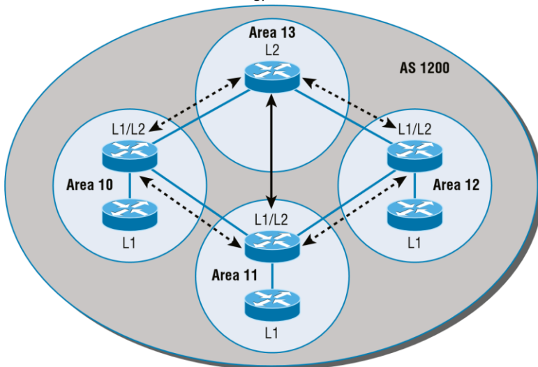
FIGURE 10.10 IS- IS network terminology
