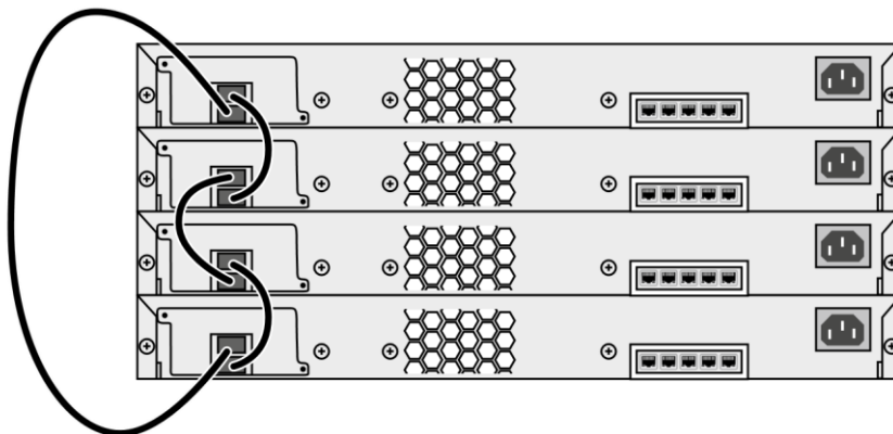
FIGURE 15.4 Switch stacking
