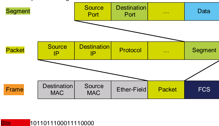
FIGURE 6.22 PDU and layer addressing
