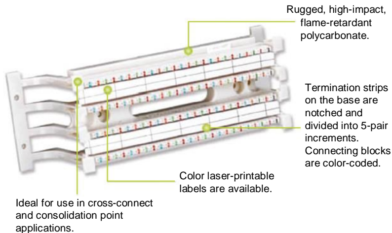
FIGURE 3.27 A 110 block
